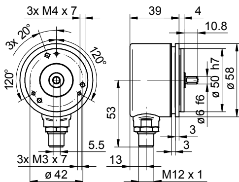
EAM580, synchro flange with M12
