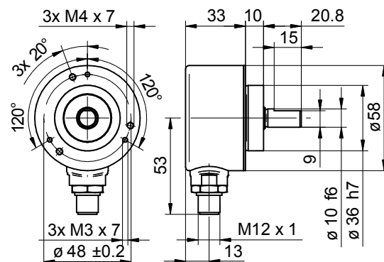
EAM580, clamping flange with M12
