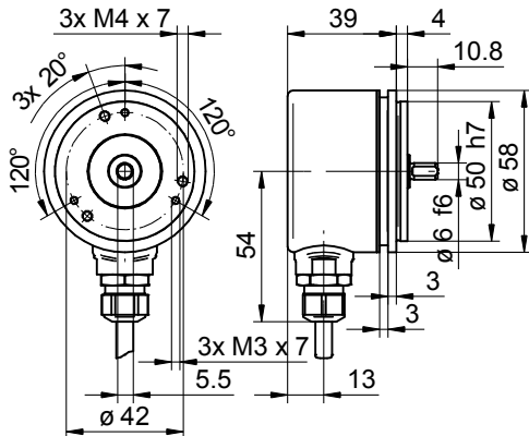
EAM580, synchro flange with cable
