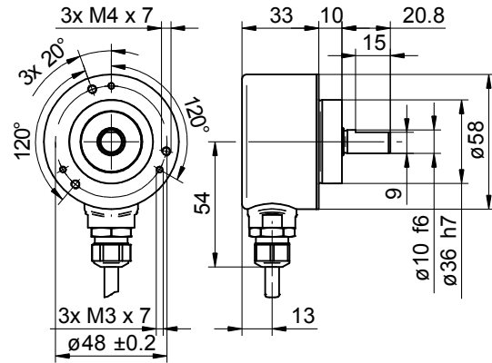
EAM580, clamping flange with cable
